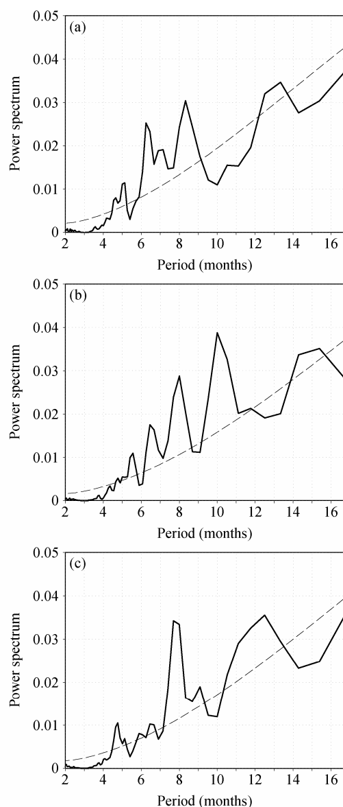
图 11 极涡振荡指数连续功率谱分析: (a) NCEP; (b) SAMIL; (c) BCC_AGCM。虚线: 95%信度红噪声标准谱 Fig. 11 Continuous spectrums of the polar vortex oscillation indices: (a) NCEP; (b) SAMIL; (c) BCC_AGCM. Dashed line: 95% confidence level red noise spectrum
