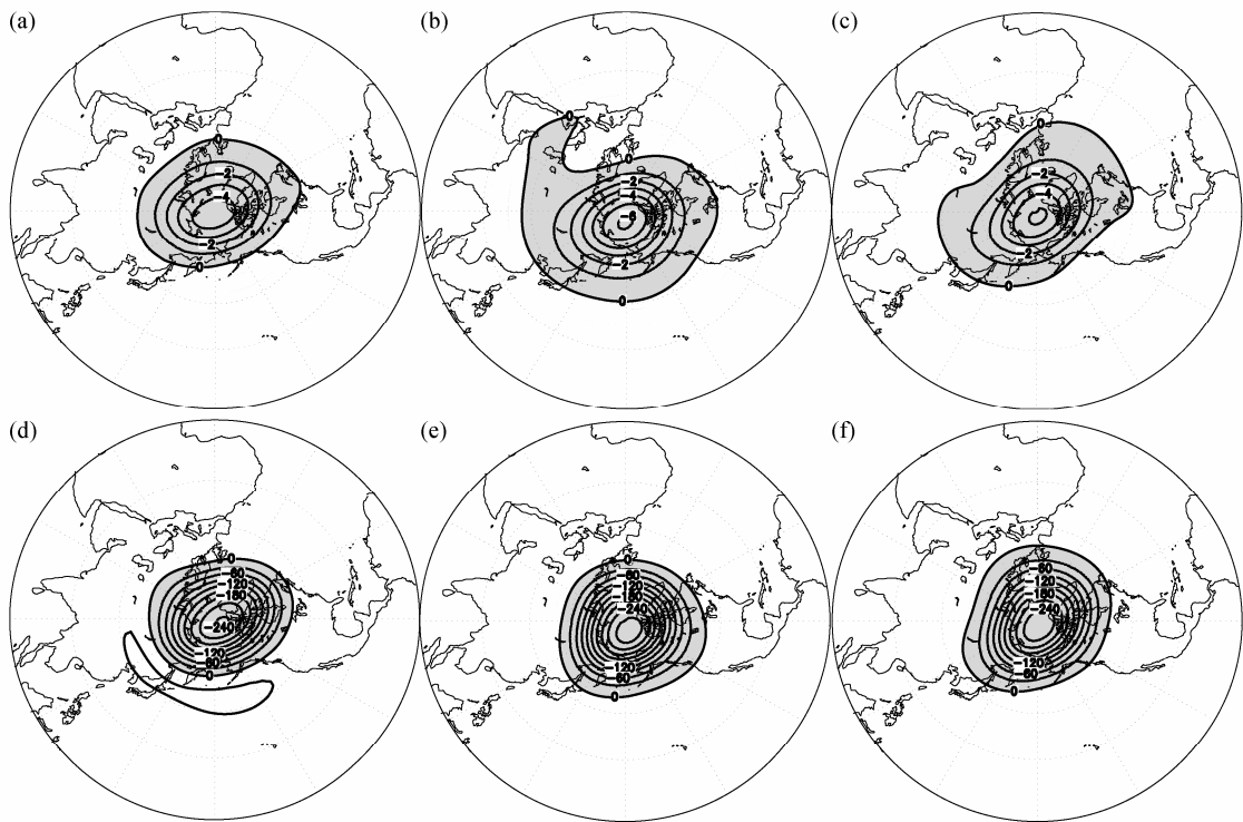
图 8 用极涡振荡指数回归的 100~20 hPa 水平温度异常场 (a、b、c; 单位: K) 和位势高度场异常场 (d、e、f; 单位: gpm) 分布: (a、d) NCEP; (b、e) SAMIL; (c、f) BCC_AGCM。阴影: 负值区域 Fig. 8 Regressions of (a, b, c) temperature anomalies (K) and (d, e, f) geopotential height anomalies (gpm) averaged for 100–20 hPa against the corresponding polar vortex oscillation indices: (a, d) NCEP; (b, e) SAMIL; (c, f) BCC_AGCM. Shaded areas: negatives
