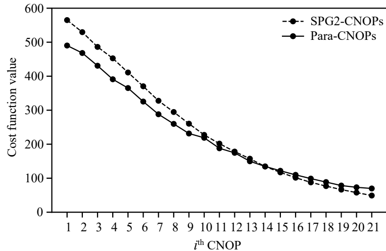
Fig. 8. Values of the cost function for SPG2-CNOPs (dashed line) and Para-CNOPs (solid line), which are averaged for 200 truth runs.
